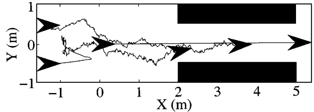
Fig. 6. Formation change for three robots in the presence of sensory noise.
