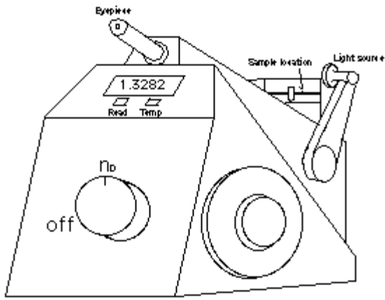
Figure 2. Refractometer used to measure methanol/ethanol concentrations
