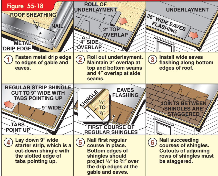
Figure 55-18. Drip edges, underlayment, and eaves flashing must be installed prior to installing asphalt strip shingles. In this example, three-tab strip shingles are used.
