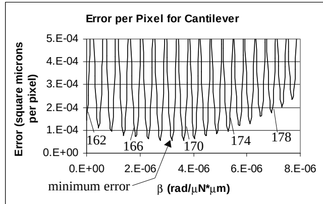
Figure 5: Error as a function of E and \beta for the 1,000 \mu\text{m} cantilever. Different values for E are labeled in GPa.
