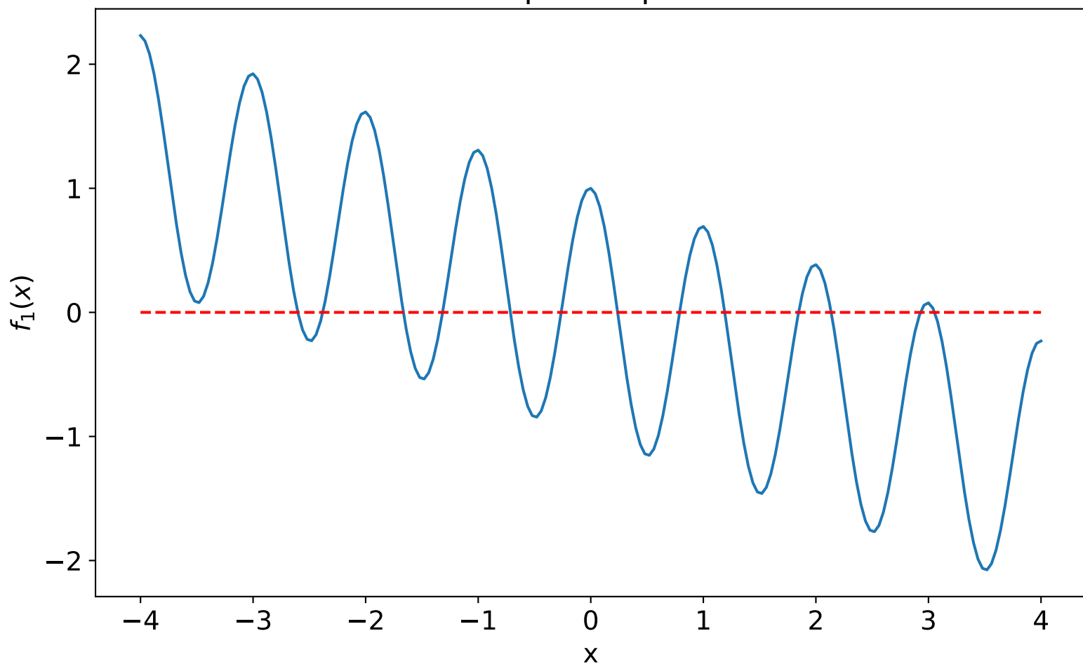
An Implicit Equation
