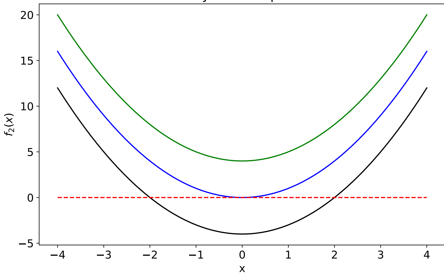
A Polynomial Equation
